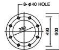
GUIDE PLATE DETAIL
