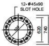
BASE PLATE DETAIL
