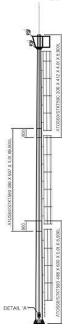
SIDE VIEW
