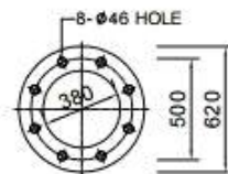
GUIDE PLATE DETAIL
