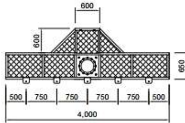
B-B' DETAIL
