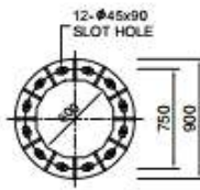
BASE PLATE DETAIL
