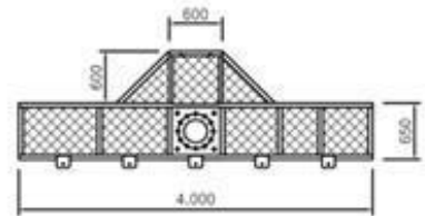
B-B' DETAIL
