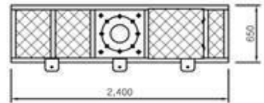
B-B' DETAIL
