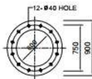
GUIDE PLATE DETAIL
