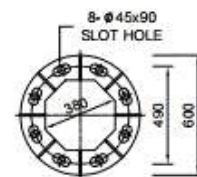
BASE PLATE DETAIL
