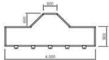
A-A' DETAIL
