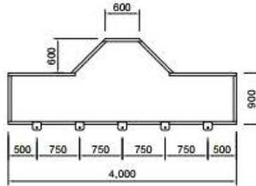
A-A' DETAIL
