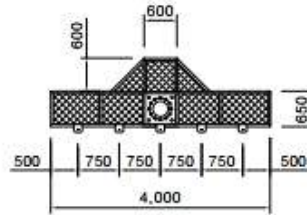
B-B DETAIL
