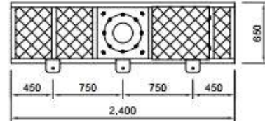
B-'B' DETAIL
