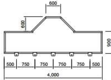
A-A' DETAIL
