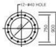
GUIDE PLATE DETAIL
