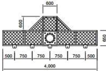
B-B' DETAIL
