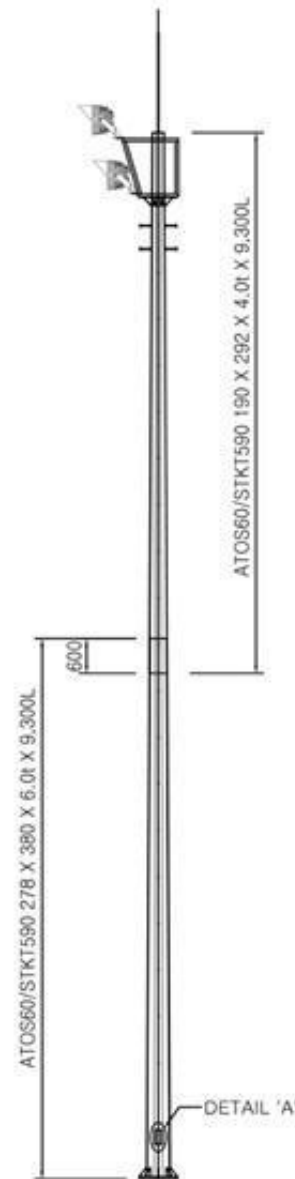
SIDE VIEW
