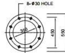
GUIDE PLATE DETAIL
