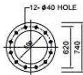
GUIDE PLATE DETAIL
