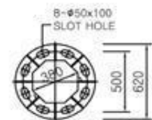
BASE PLATE DETAIL
