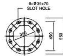
BASE PLATE DETAIL
