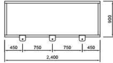
A-'A' DETAIL
